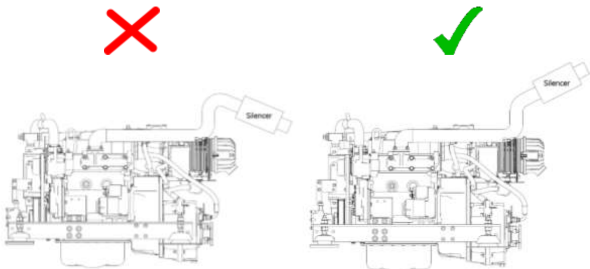
Figure 15: Correct Exhaust Installation
