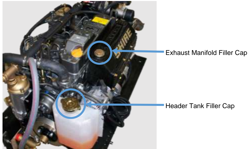
Figure 14: Shire 50 Coolant Filling Points
